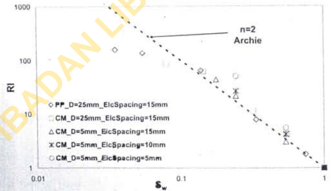
Figure 8: RI- S_w for Bentheim Sandstone.
