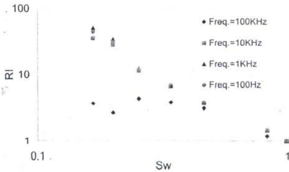
Figure 4: RI- S_w for Berea Sandstone.
