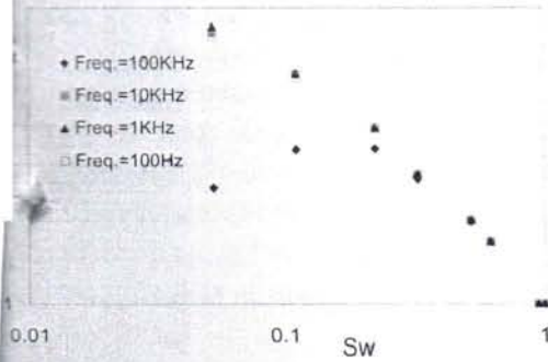
Figure 6: RI- S_w for Mount Gambier Carbonate.
