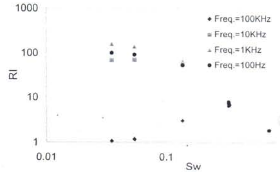
Figure 5: RI- S_w for Bentheim Sandstone.
