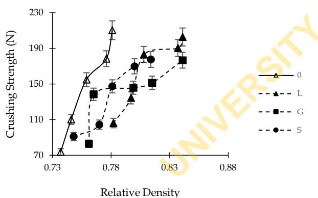
Fig. 2. The plots of crushing strength versus relative density of paracetamol tablets containing 0 and 10 %w/w of the yam starch (Lagos, L; Giwa, G, and Sule, S) disintegrants.
