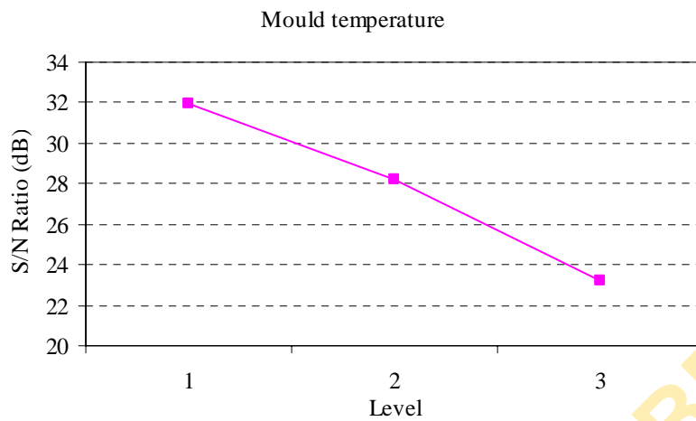
Figure 2a. Main effects plot for mould temperature S/N ratio values on impact energy
